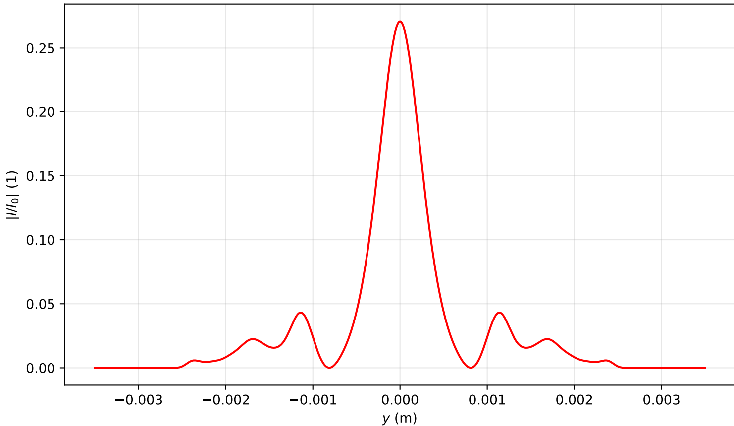
Intensity profile I(x = 0, y, z = 3.821)/I_0 , \text{Pin}=8.0\text{Pcr} , artificial time
